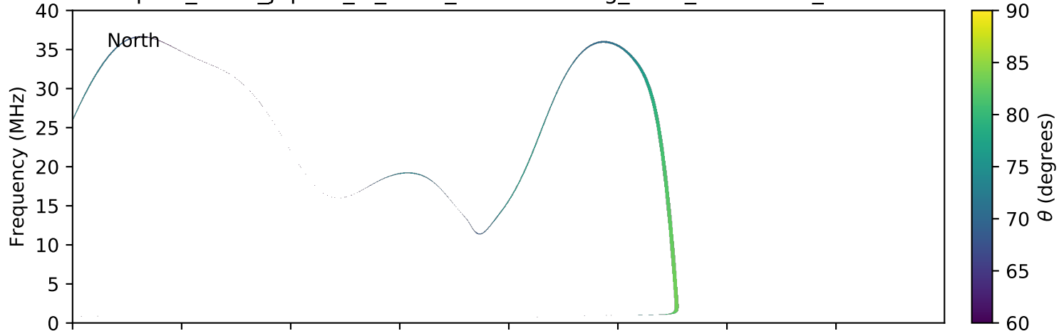
expres_earth_jupiter_io_isaac_lossc-wid1deg_3kev_20150927_v01.cdf
