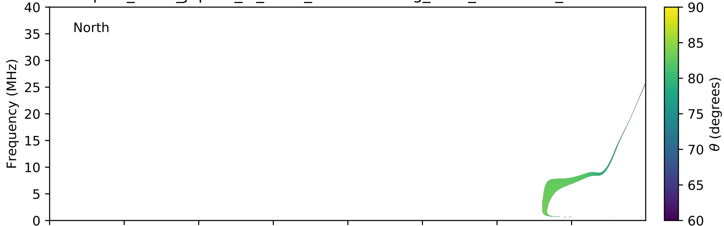
expres_earth_jupiter_io_isaac_lossc-wid1deg_3kev_20150926_v01.cdf
