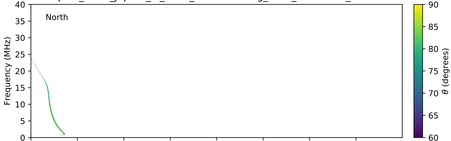
expres_earth_jupiter_io_isaac_lossc-wid1deg_3kev_20150924_v01.cdf
