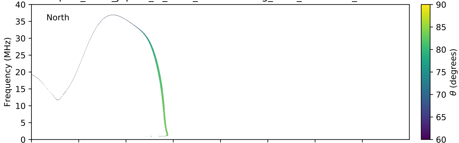
expres_earth_jupiter_io_isaac_lossc-wid1deg_3kev_20150922_v01.cdf
