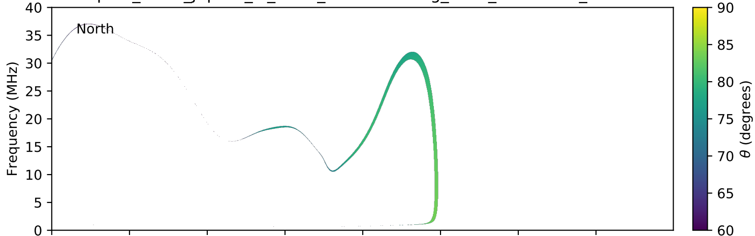
expres_earth_jupiter_io_isaac_lossc-wid1deg_3kev_20150920_v01.cdf
