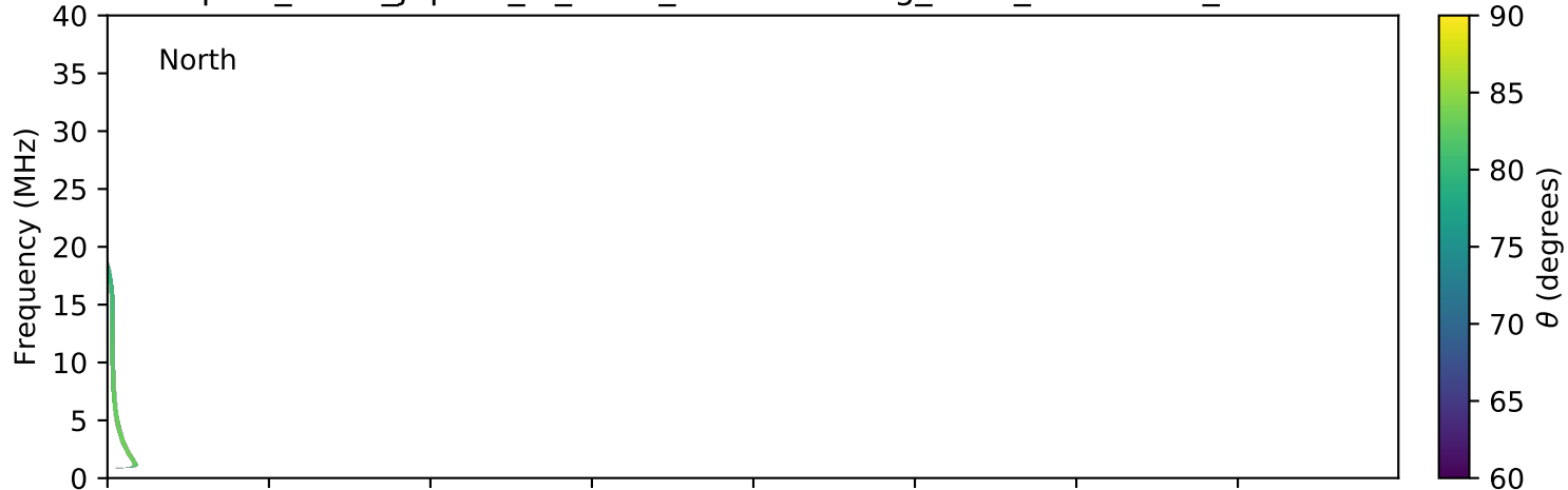
expres_earth_jupiter_io_isaac_lossc-wid1deg_3kev_20150917_v01.cdf
