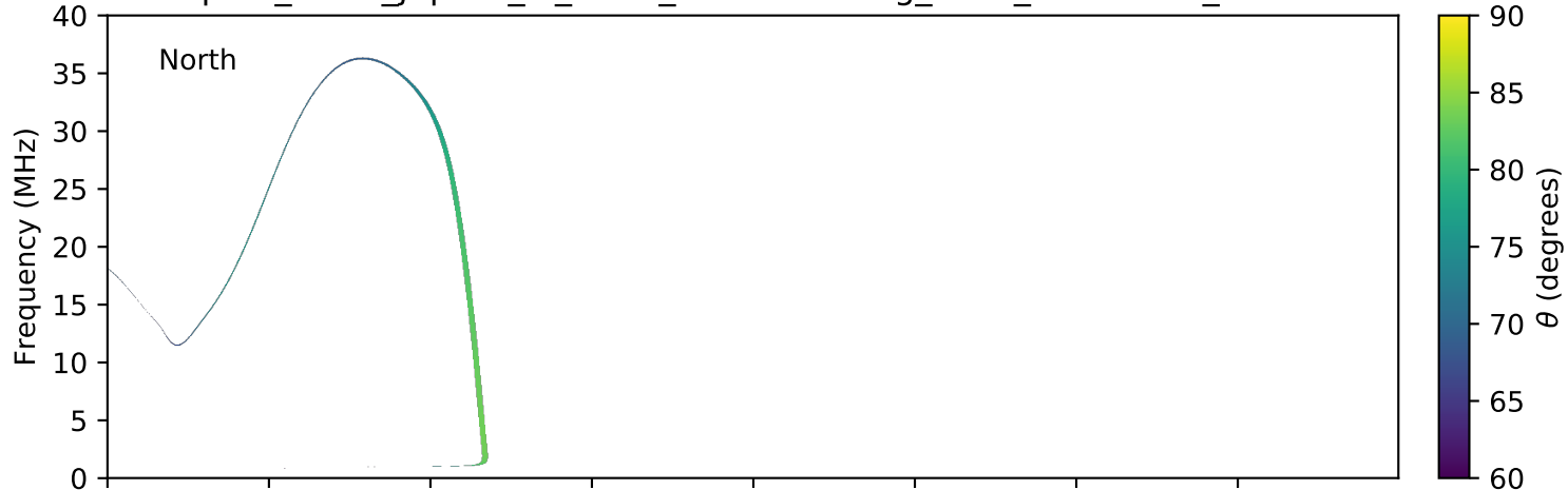
expres_earth_jupiter_io_isaac_lossc-wid1deg_3kev_20150915_v01.cdf
