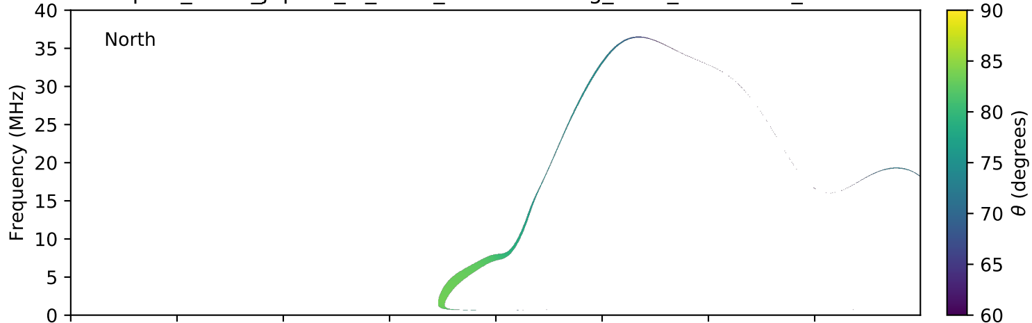
expres_earth_jupiter_io_isaac_lossc-wid1deg_3kev_20150914_v01.cdf
