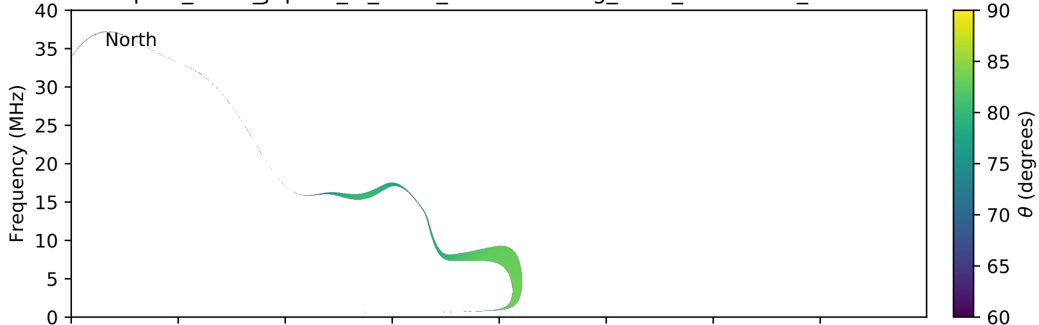
expres_earth_jupiter_io_isaac_lossc-wid1deg_3kev_20150913_v01.cdf
