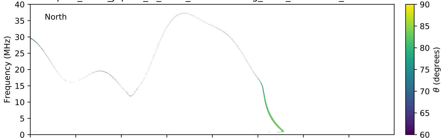
expres_earth_jupiter_io_isaac_lossc-wid1deg_3kev_20150911_v01.cdf
