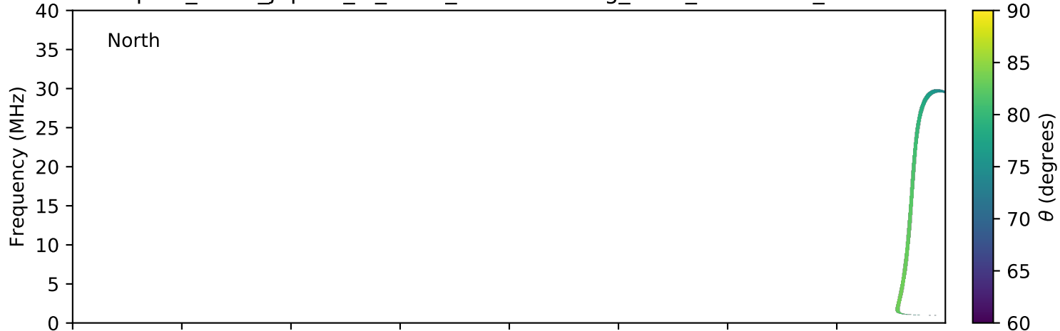
expres_earth_jupiter_io_isaac_lossc-wid1deg_3kev_20150910_v01.cdf
