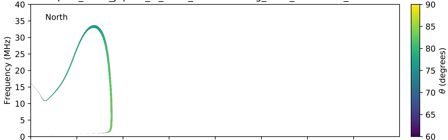
expres_earth_jupiter_io_isaac_lossc-wid1deg_3kev_20150908_v01.cdf
