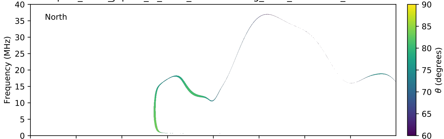
expres_earth_jupiter_io_isaac_lossc-wid1deg_3kev_20150907_v01.cdf
