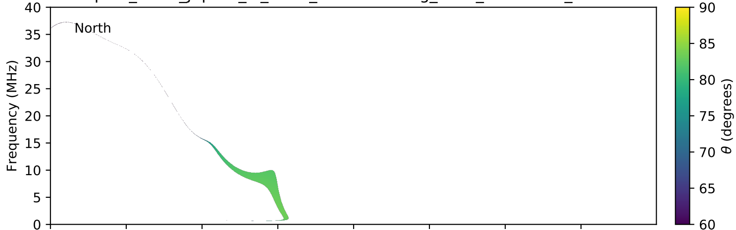
expres_earth_jupiter_io_isaac_lossc-wid1deg_3kev_20150906_v01.cdf
