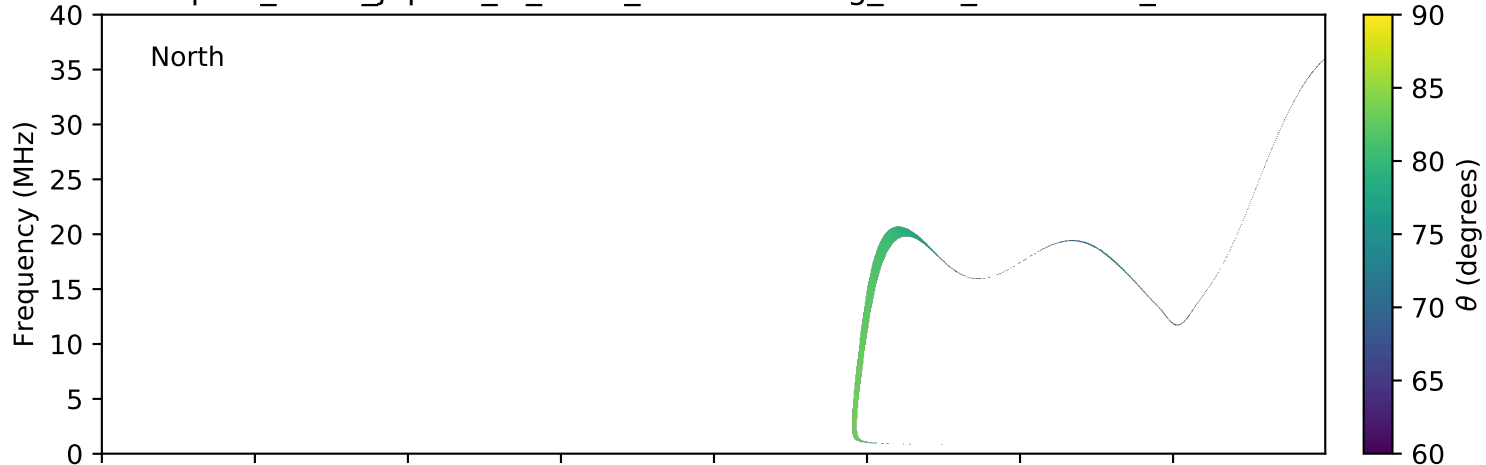
expres_earth_jupiter_io_isaac_lossc-wid1deg_3kev_20150905_v01.cdf
