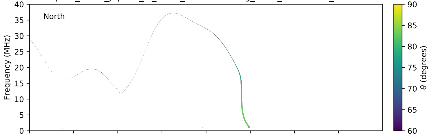
expres_earth_jupiter_io_isaac_lossc-wid1deg_3kev_20150904_v01.cdf
