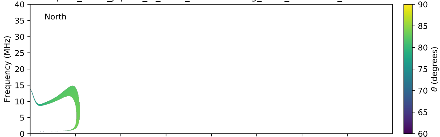
expres_earth_jupiter_io_isaac_lossc-wid1deg_3kev_20150901_v01.cdf
