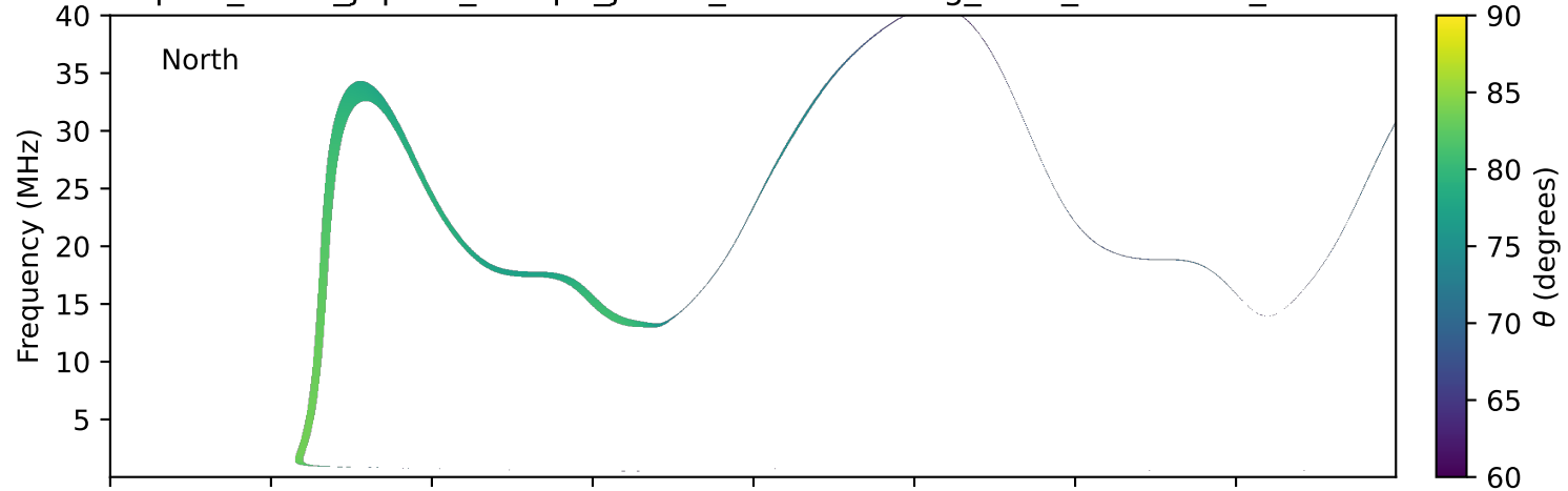
expres_earth_jupiter_europa_jrm33_lossc-wid1deg_3kev_20150917_v11.cdf
