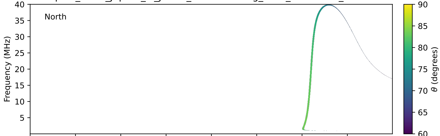
expres_earth_jupiter_io_jrm33_lossc-wid1deg_3kev_20150830_v11.cdf
