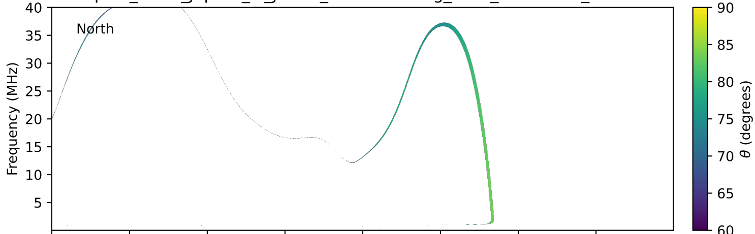
expres_earth_jupiter_io_jrm33_lossc-wid1deg_3kev_20150822_v11.cdf
