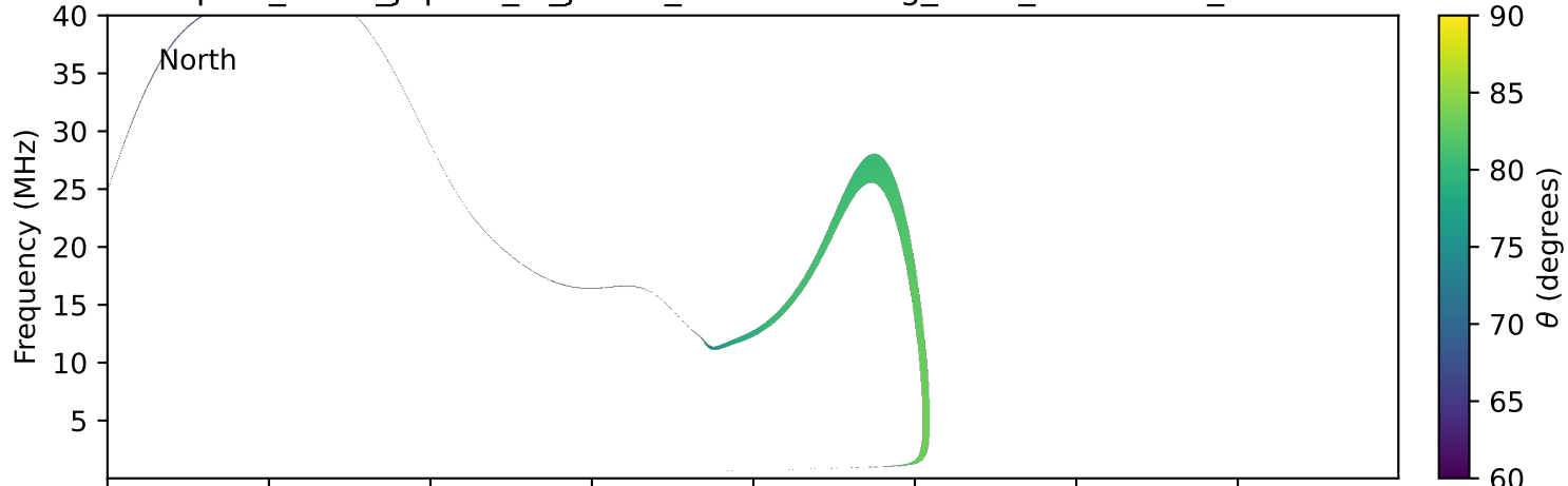
expres_earth_jupiter_io_jrm33_lossc-wid1deg_3kev_20150815_v11.cdf
