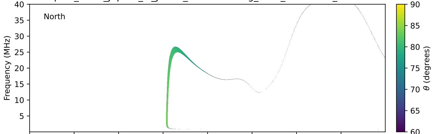
expres_earth_jupiter_io_jrm33_lossc-wid1deg_3kev_20150811_v11.cdf
