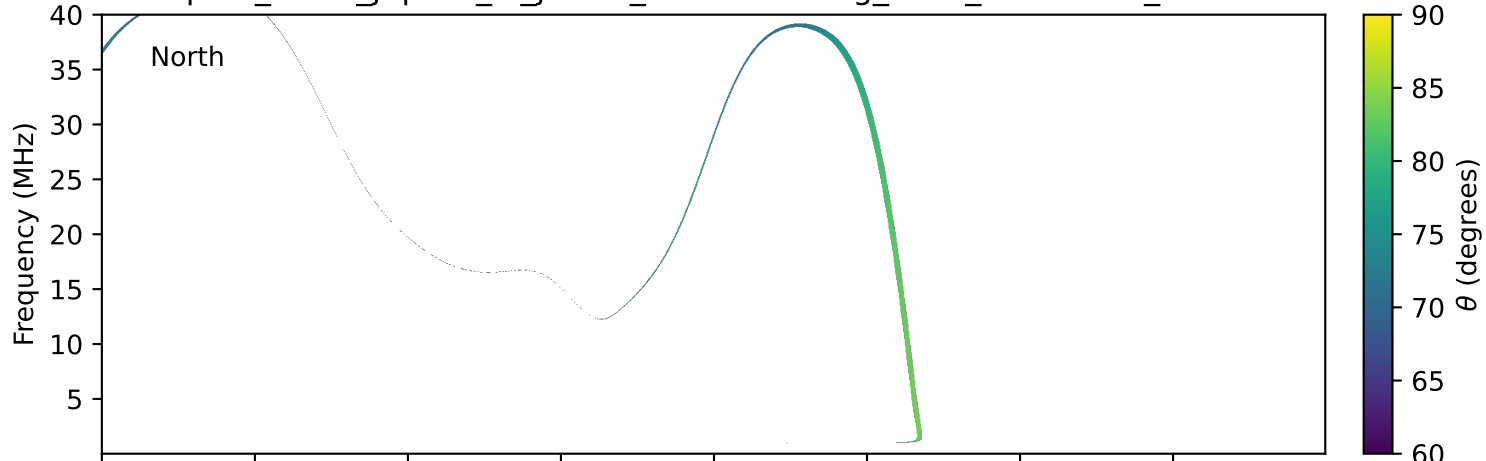
expres_earth_jupiter_io_jrm33_lossc-wid1deg_3kev_20150808_v11.cdf
