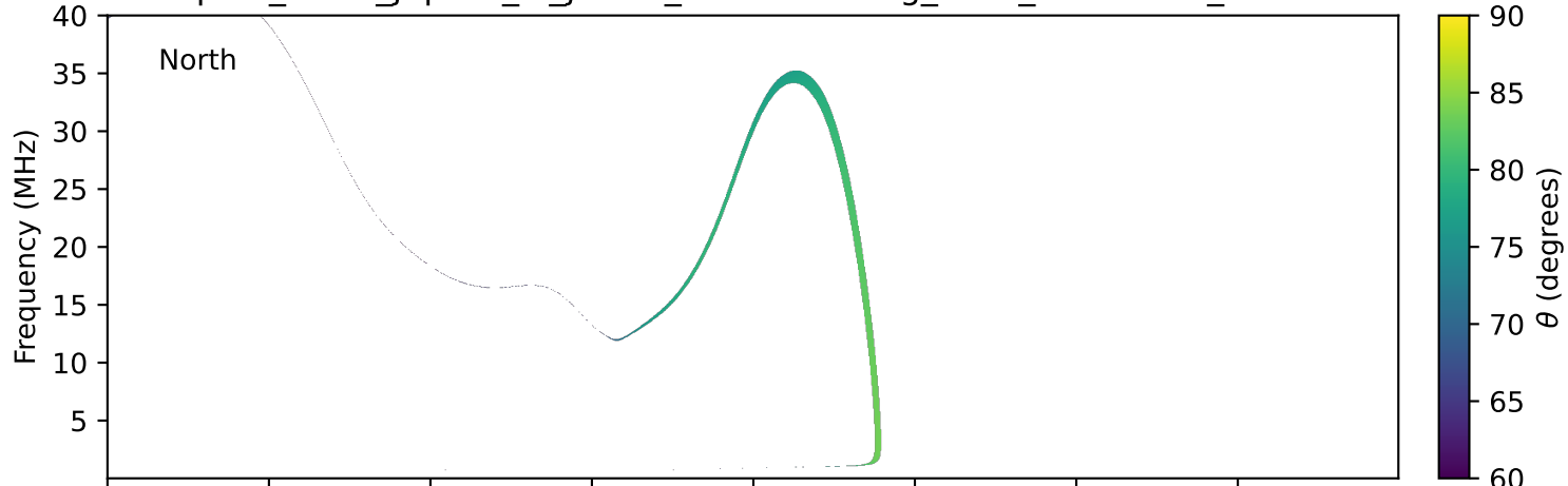
expres_earth_jupiter_io_jrm33_lossc-wid1deg_3kev_20150801_v11.cdf
