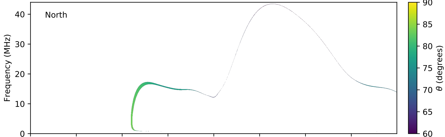
expres_earth_jupiter_io_jrm09_lossc-wid1deg_3kev_20150831_v01.cdf
