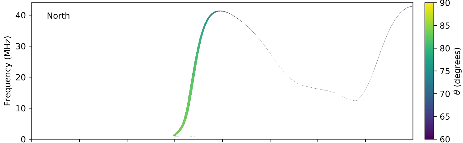
expres_earth_jupiter_io_jrm09_lossc-wid1deg_3kev_20150815_v01.cdf
