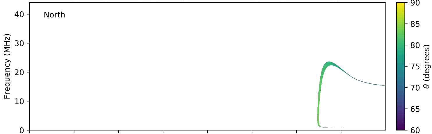
expres_earth_jupiter_io_jrm09_lossc-wid1deg_3kev_20150811_v01.cdf
