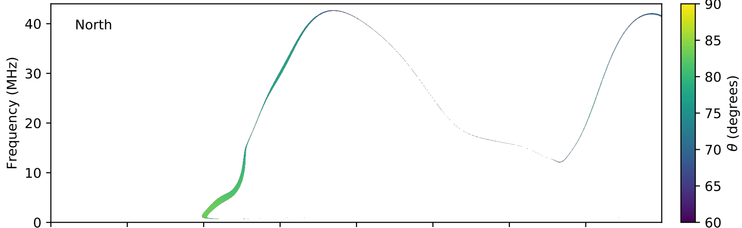
expres_earth_jupiter_io_jrm09_lossc-wid1deg_3kev_20150808_v01.cdf
