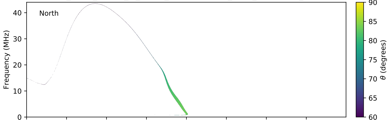
expres_earth_jupiter_io_jrm09_lossc-wid1deg_3kev_20150805_v01.cdf
