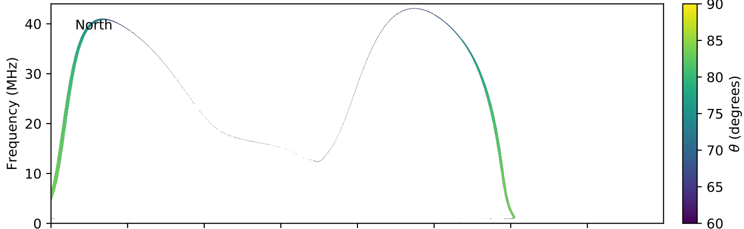
expres_earth_jupiter_io_jrm09_lossc-wid1deg_3kev_20150803_v01.cdf
