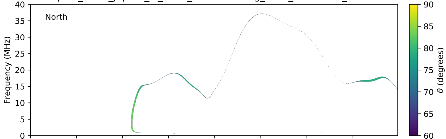
expres_earth_jupiter_io_isaac_lossc-wid1deg_3kev_20150831_v01.cdf
