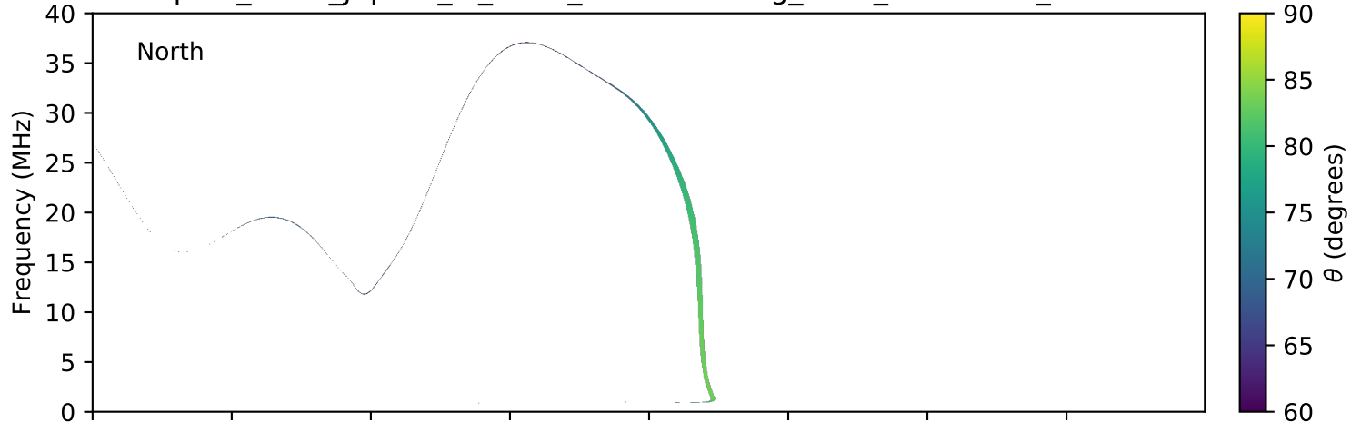
expres_earth_jupiter_io_isaac_lossc-wid1deg_3kev_20150828_v01.cdf
