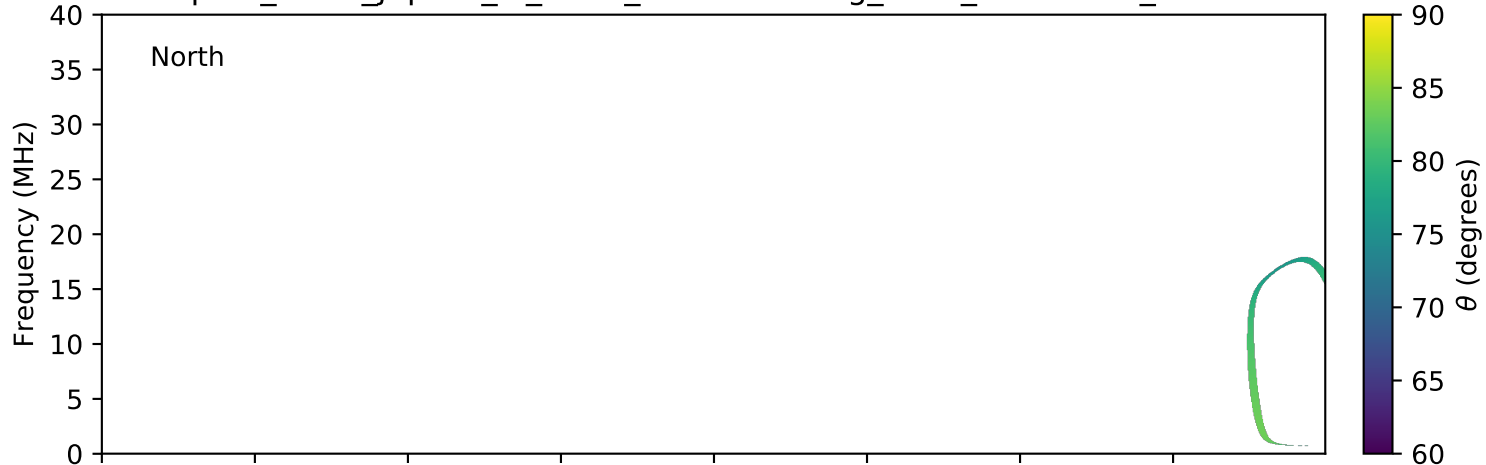
expres_earth_jupiter_io_isaac_lossc-wid1deg_3kev_20150825_v01.cdf
