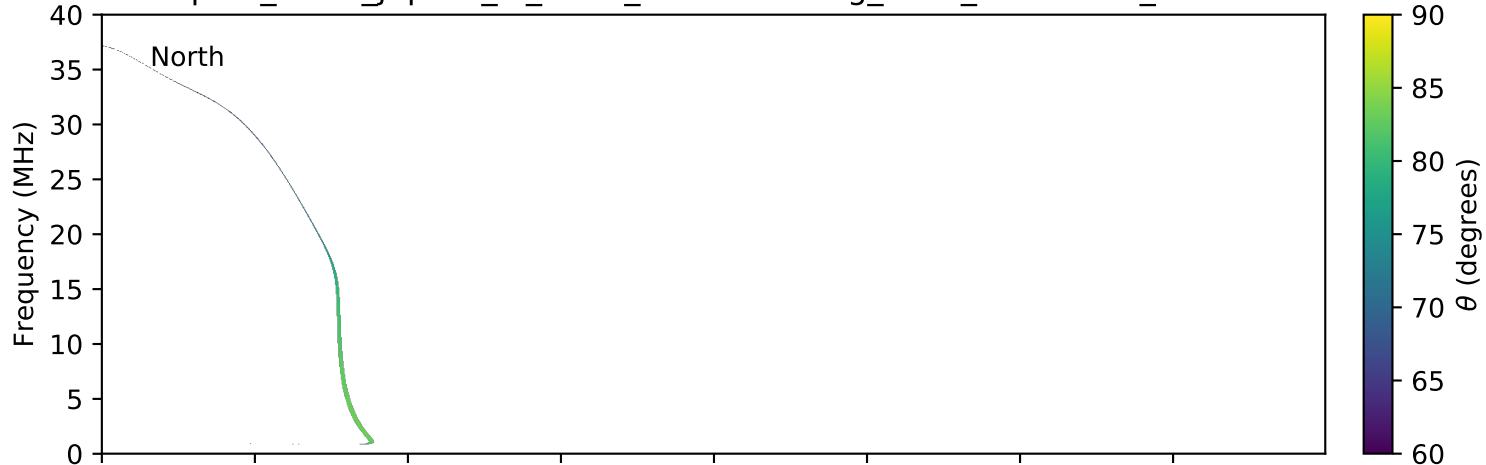
expres_earth_jupiter_io_isaac_lossc-wid1deg_3kev_20150823_v01.cdf
