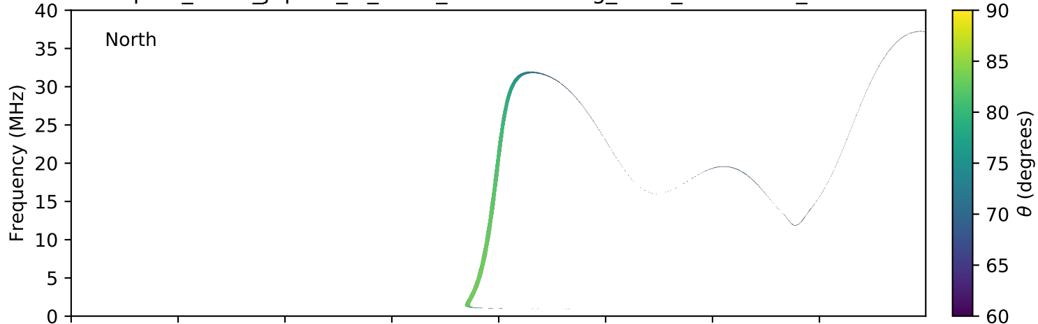
expres_earth_jupiter_io_isaac_lossc-wid1deg_3kev_20150822_v01.cdf
