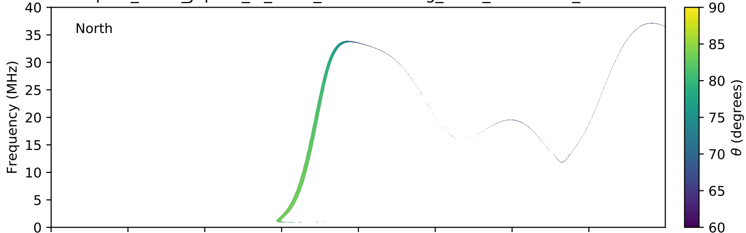
expres_earth_jupiter_io_isaac_lossc-wid1deg_3kev_20150815_v01.cdf
