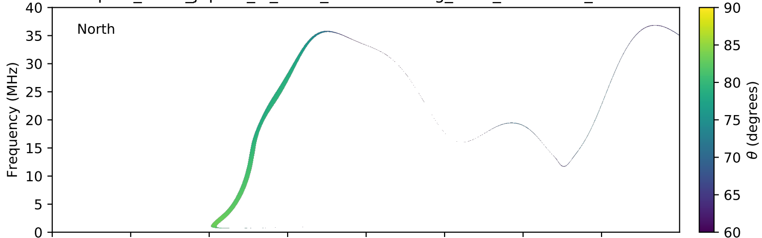
expres_earth_jupiter_io_isaac_lossc-wid1deg_3kev_20150808_v01.cdf
