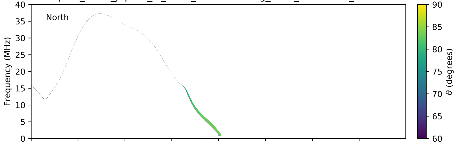
expres_earth_jupiter_io_isaac_lossc-wid1deg_3kev_20150805_v01.cdf
