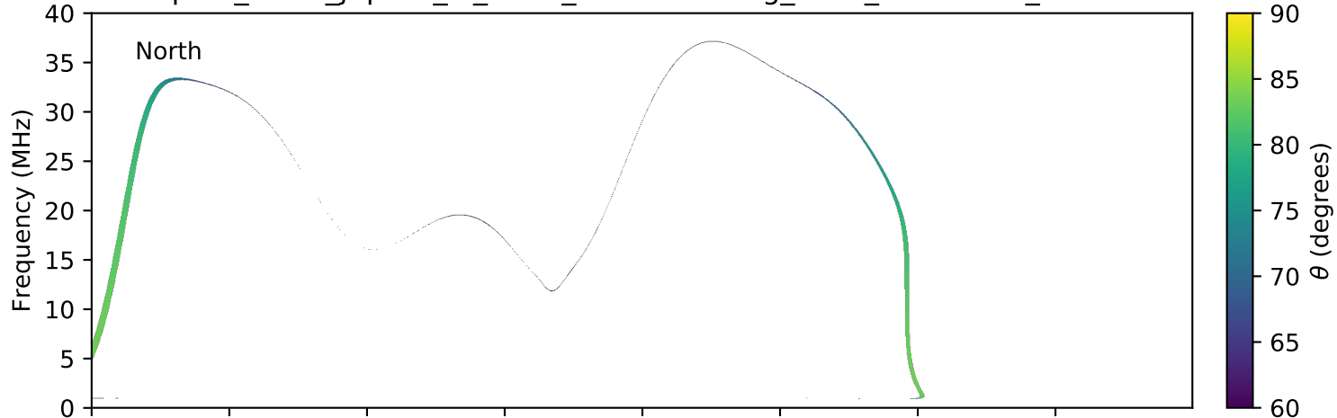
expres_earth_jupiter_io_isaac_lossc-wid1deg_3kev_20150803_v01.cdf
