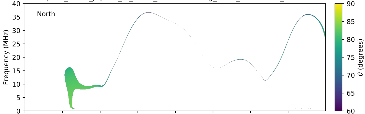
expres_earth_jupiter_io_isaac_lossc-wid1deg_3kev_20150801_v01.cdf
