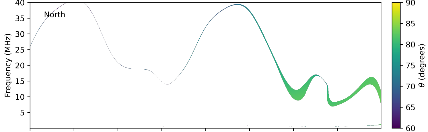
expres_earth_jupiter_europa_jrm33_lossc-wid1deg_3kev_20150820_v11.cdf
