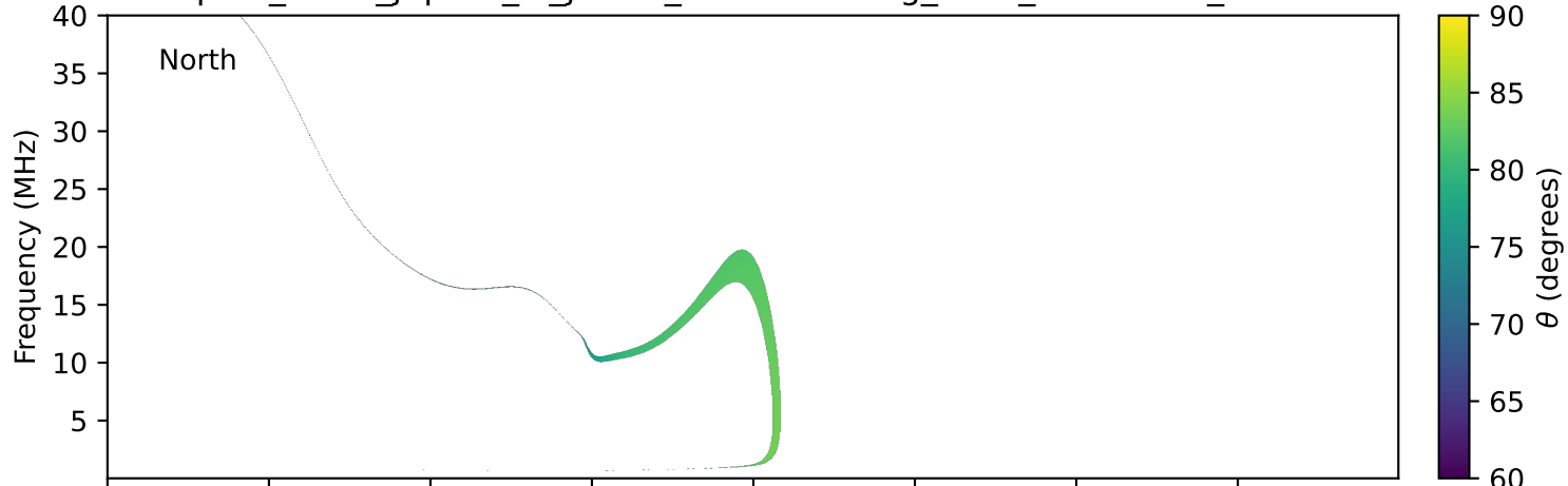
expres_earth_jupiter_io_jrm33_lossc-wid1deg_3kev_20150725_v11.cdf
