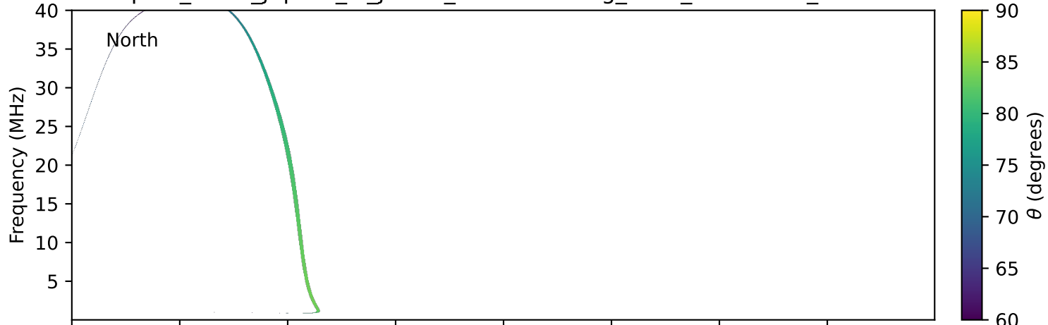
expres_earth_jupiter_io_jrm33_lossc-wid1deg_3kev_20150720_v11.cdf
