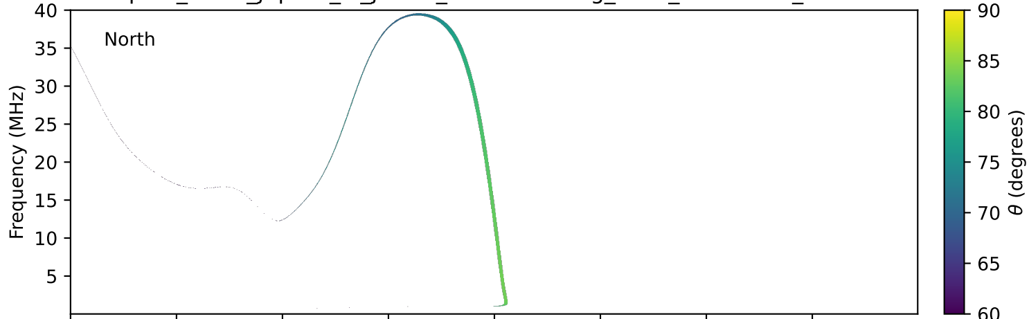
expres_earth_jupiter_io_jrm33_lossc-wid1deg_3kev_20150704_v11.cdf
