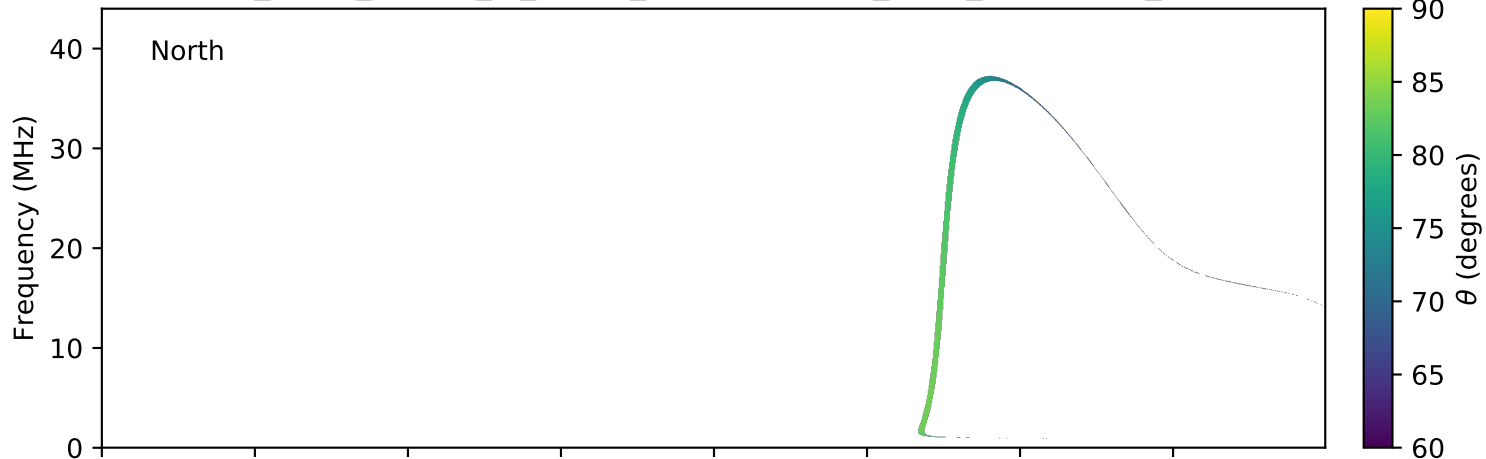
expres_earth_jupiter_io_jrm09_lossc-wid1deg_3kev_20150728_v01.cdf
