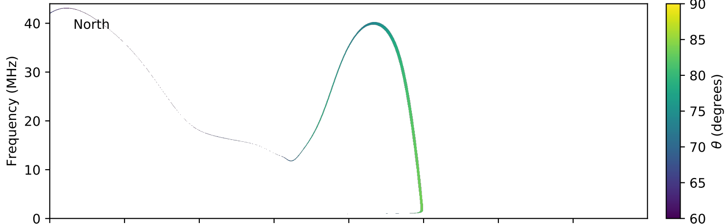
expres_earth_jupiter_io_jrm09_lossc-wid1deg_3kev_20150720_v01.cdf
