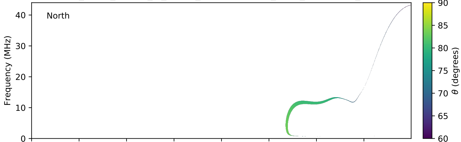
expres_earth_jupiter_io_jrm09_lossc-wid1deg_3kev_20150712_v01.cdf
