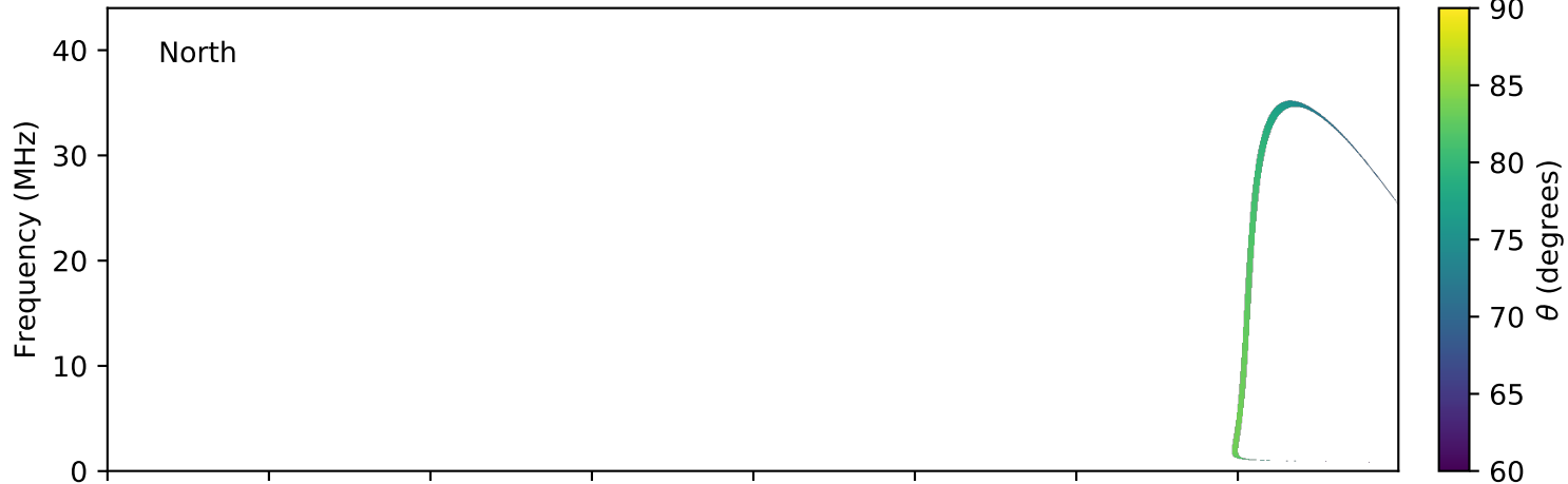
expres_earth_jupiter_io_jrm09_lossc-wid1deg_3kev_20150703_v01.cdf
