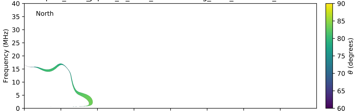
expres_earth_jupiter_io_isaac_lossc-wid1deg_3kev_20150731_v01.cdf
