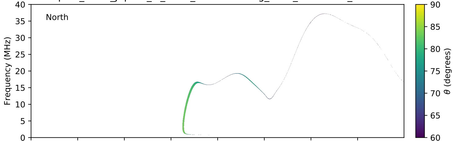
expres_earth_jupiter_io_isaac_lossc-wid1deg_3kev_20150730_v01.cdf
